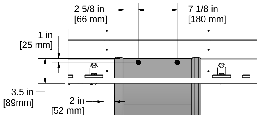
DRILLING LOCATIONS
