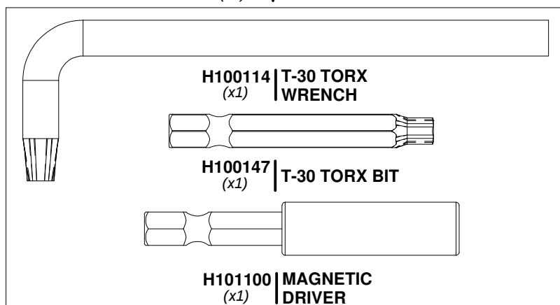
9220119 | TOOL KIT (x1)
