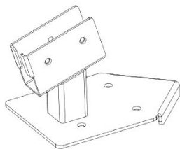
A4M01234 POST CLIP ASSEMBLY (x4)
