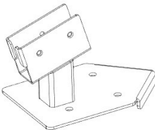
A4M01234 POST CLIP ASSEMBLY (x4)
