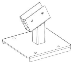
A4M01894 MIDDLE POST CLIP ASSEMBLY (x2)
